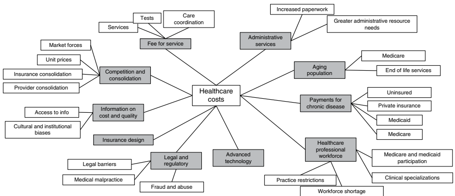
Figure 8.7. Example context diagram of healthcare costs. Source: Derived from Bipartisan Policy Center (2012).
