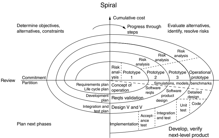
Figure 14.6. Spiral model.
