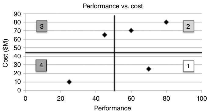
Figure 11.13. Example scatterplot of performance cost quadrants.
