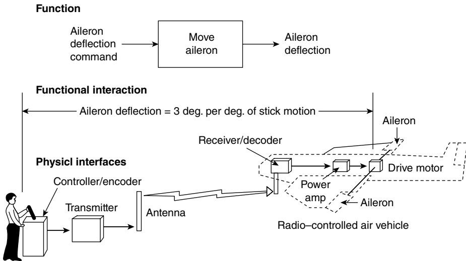
Figure 2.5. Functional interactions and physical interfaces.
