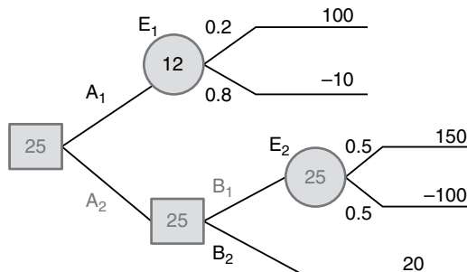
Figure 8.4. Decision tree solved.
