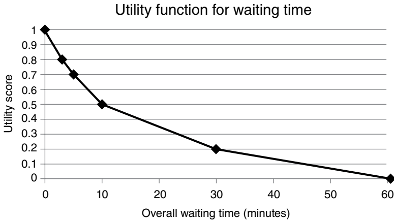
Figure 11.5. Example utility function for waiting times.
