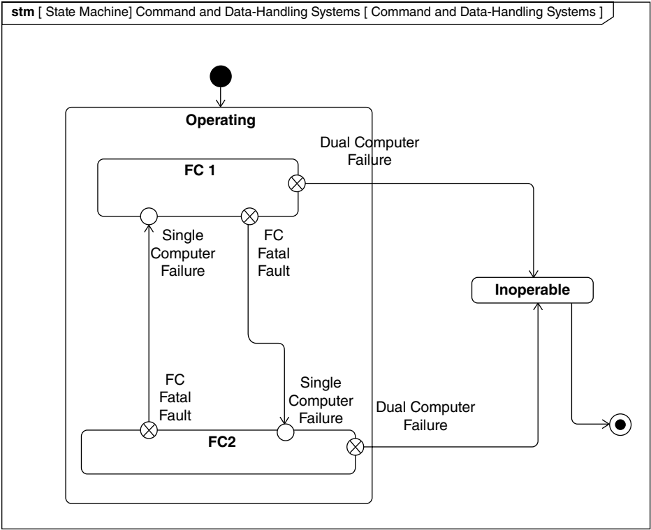
Figure 10.6. Satellite command and data-handling state machine diagram.
