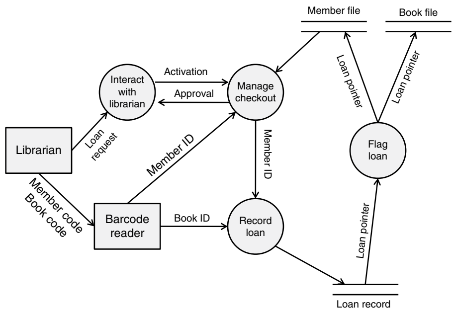
Figure 14.12. Data flow diagram: library checkout.
