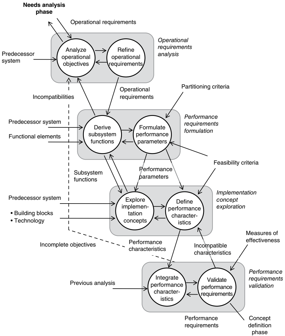
Figure 6.2. Concept exploration phase flow diagram.
