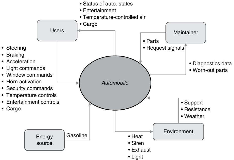
Figure 2.3. Context diagram for an automobile.
