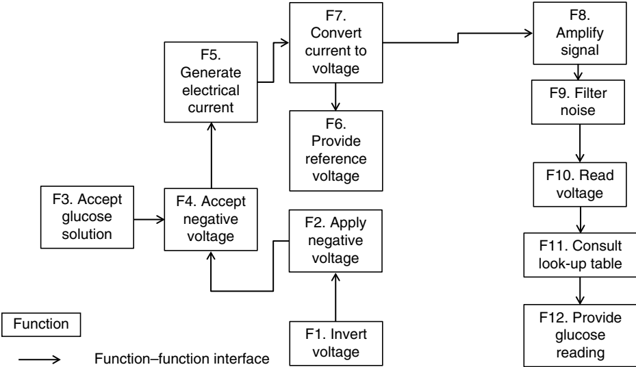
Figure 9.1. Glucose meter example functional architecture.
