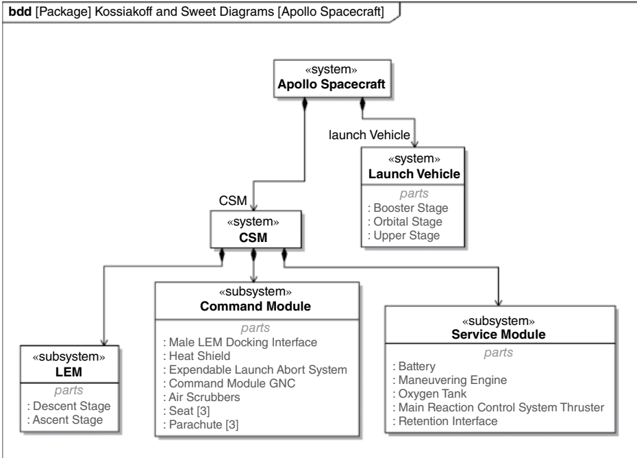
Figure 10.1. SysML block definition diagram of NASA's Apollo spacecraft.
