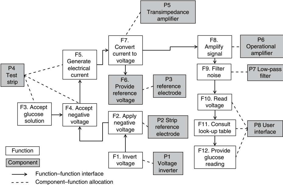
Figure 9.3. Glucose meter example allocated architecture.
