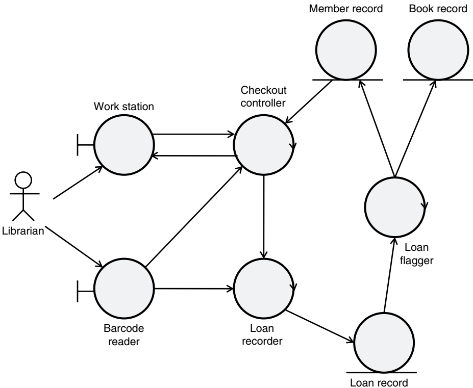
Figure 14.13. Robustness diagram: library checkout.
