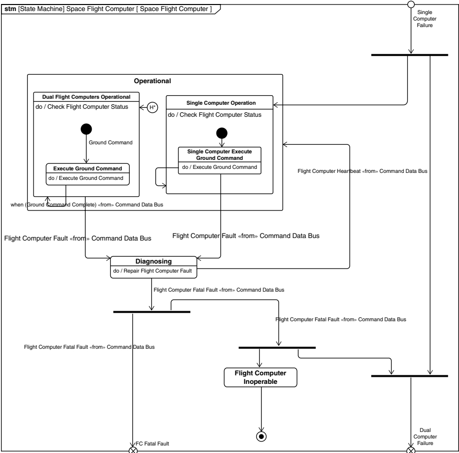
Figure 10.7. Flight computer SysML state machine.
