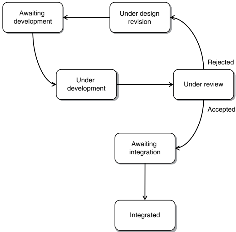
Figure 14.7. State transition diagram in concurrent development model.
