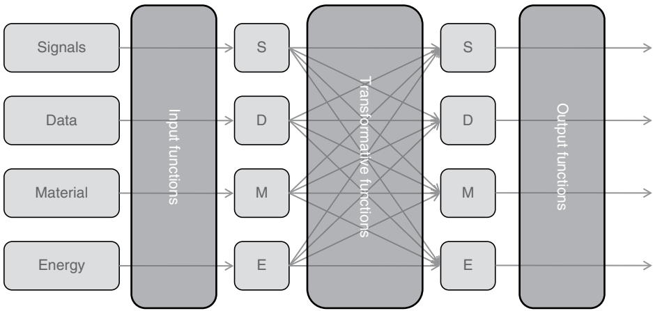
Figure 7.6. Function category vs. functional media.
