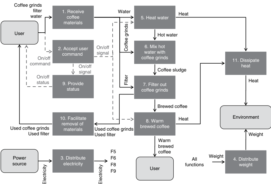
Figure 7.4. Functional block diagram of a standard coffee maker.
