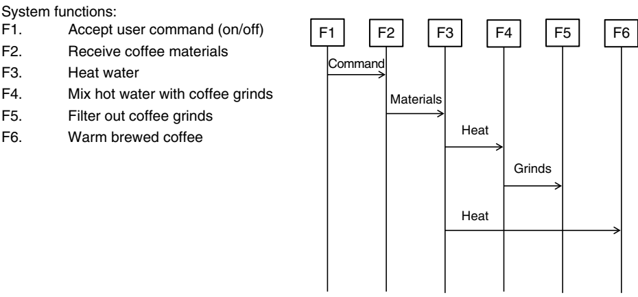
Figure 7.11. Coffee maker sequence diagram.
