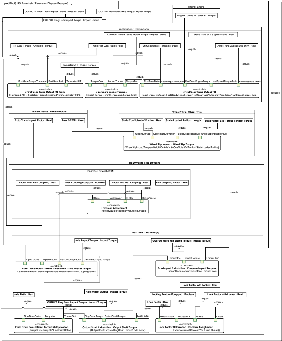
Figure 10.9. Driveline parametric diagram.
