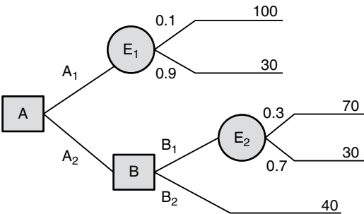
Figure 8.2. Decision tree example.
