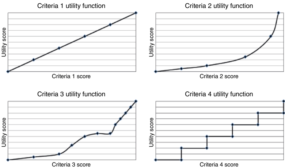
Figure 11.4. Candidate utility functions.
