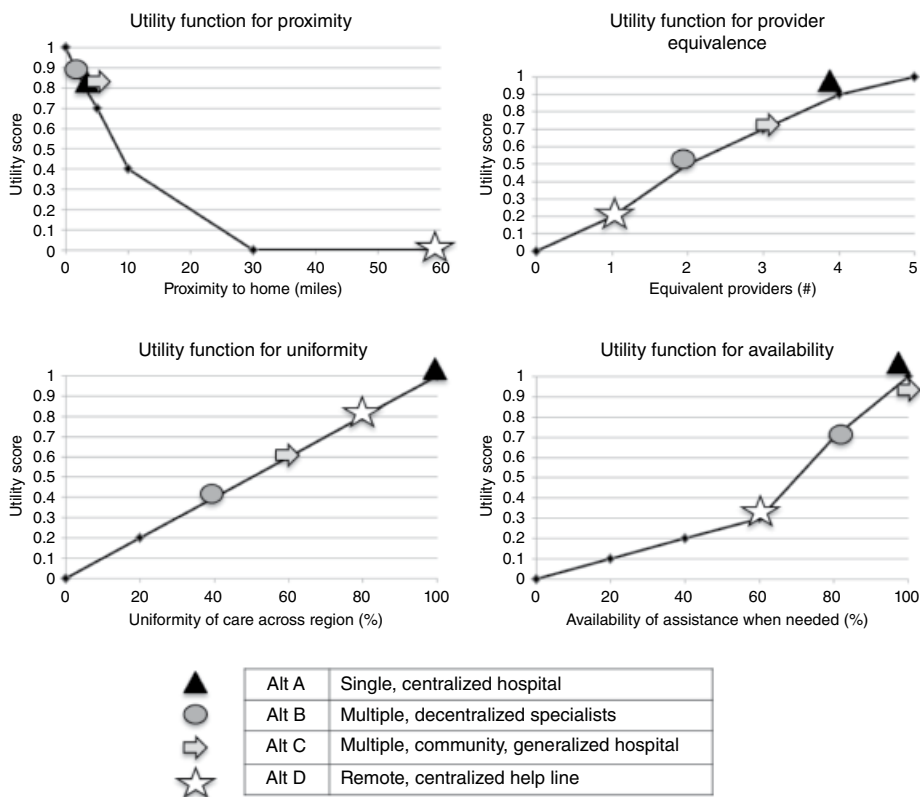
Figure 11.10. MAUT analysis example.
