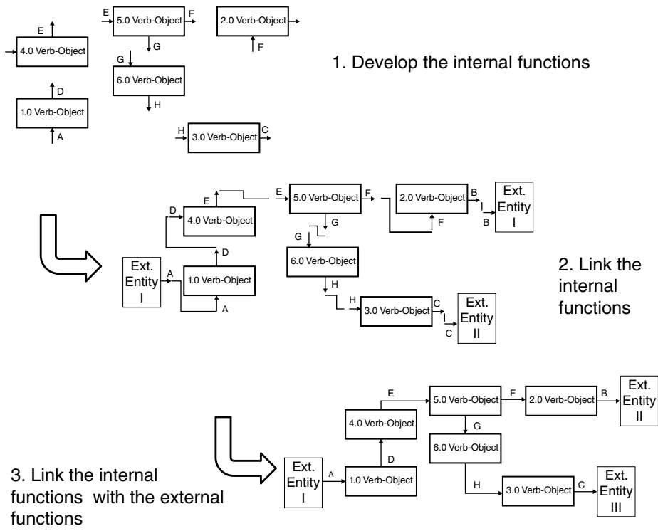
Figure 7.7. Functional block diagram development from internal view first.
