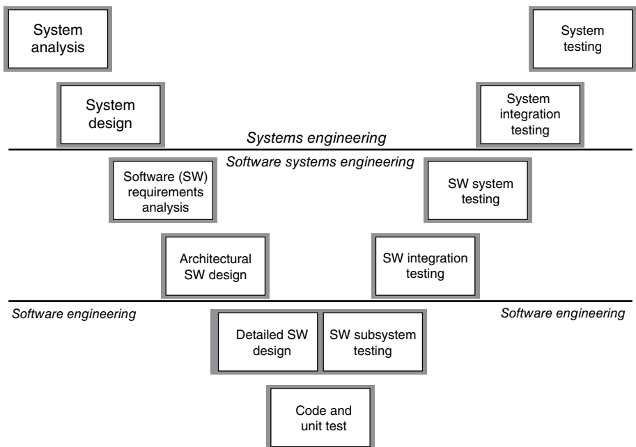
Figure 14.1. IEEE software systems engineering process.
