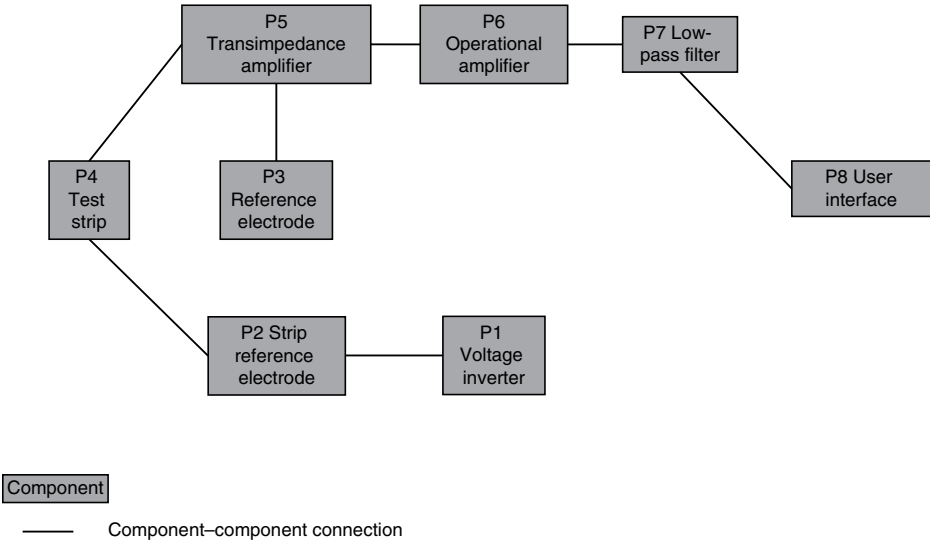
Figure 9.2. Glucose meter example physical architecture.
