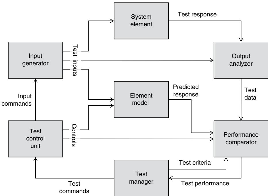
Figure 17.3. System element test configuration.
