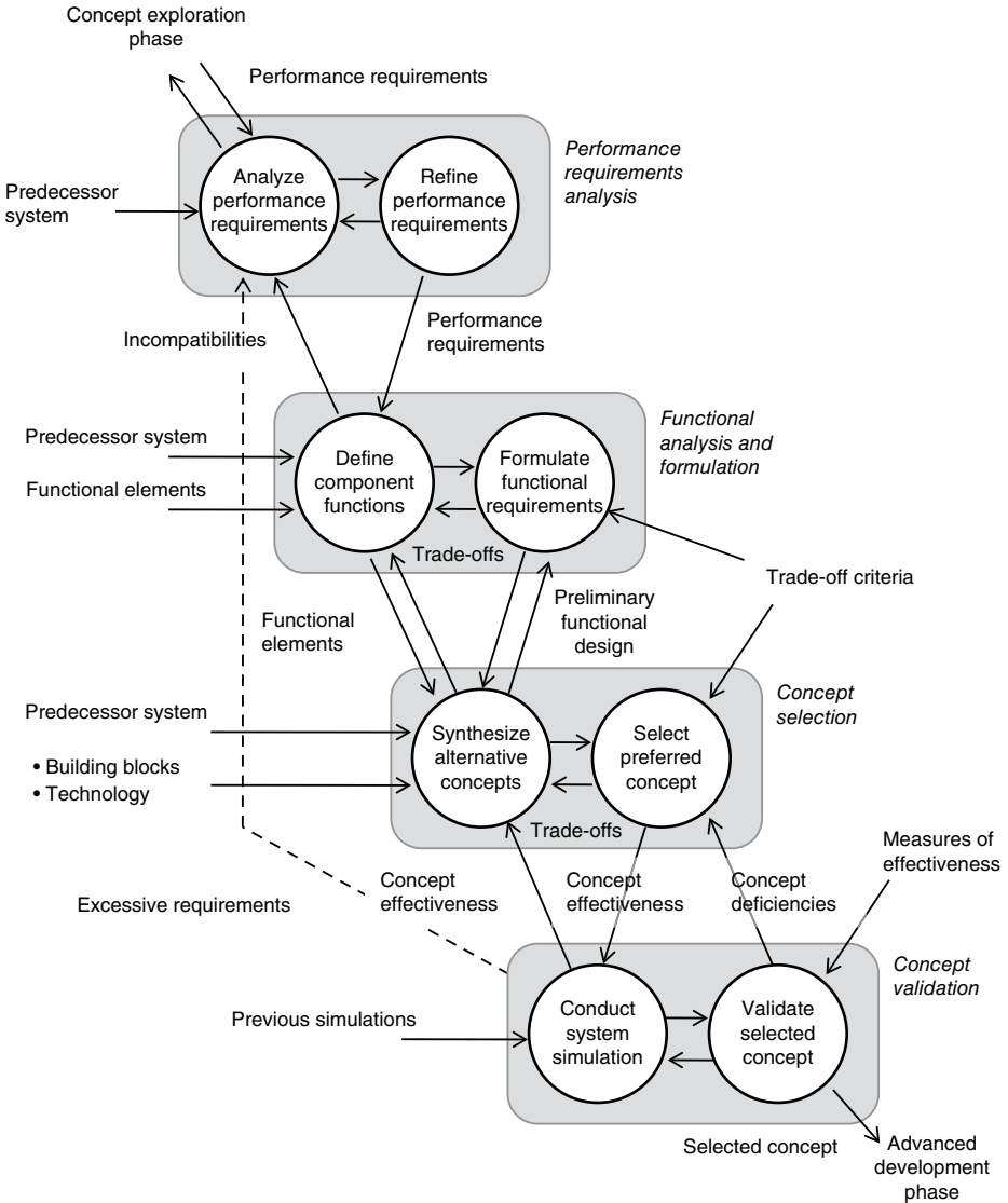
Figure 7.2. Concept definition phase flow diagram.
