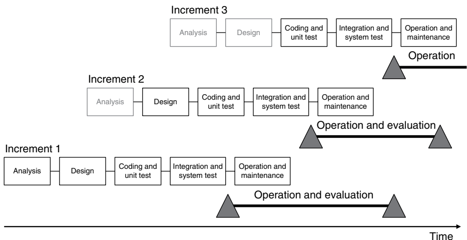
Figure 14.5. Software incremental model.
