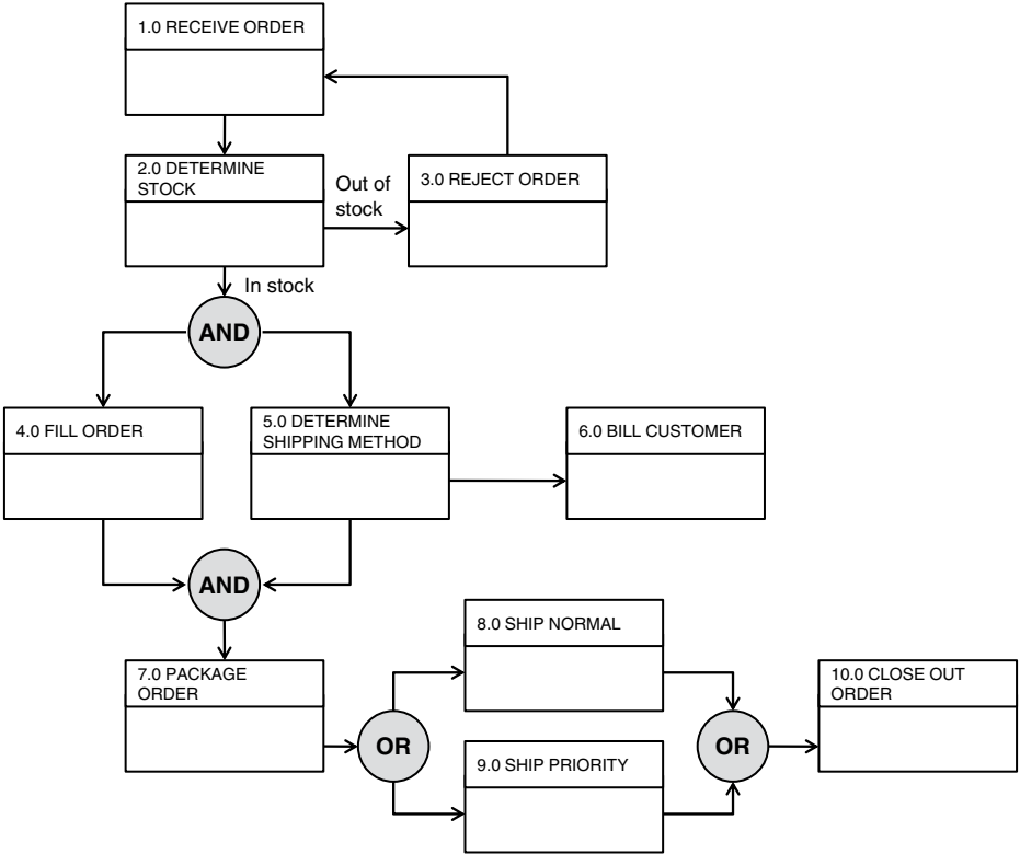
Figure 14.11. Functional flow block diagram example.
