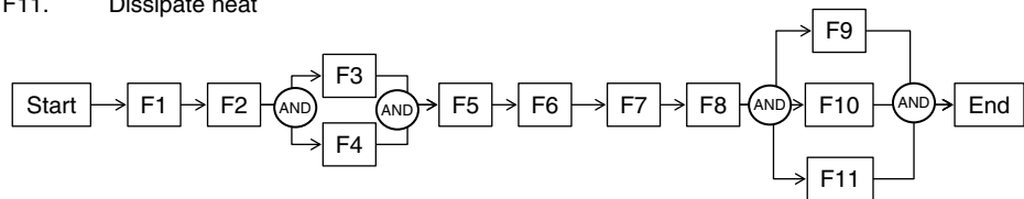
Figure 7.10. Coffee maker functional flow diagram.
