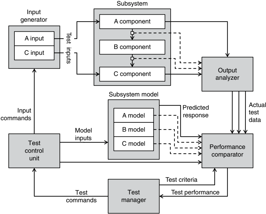
Figure 16.2. Subsystems configuration.
