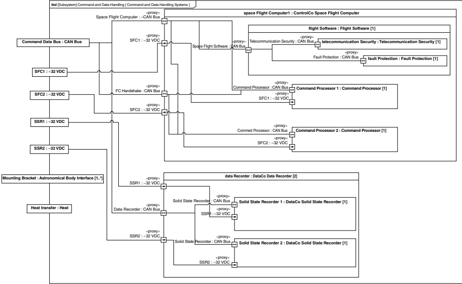
Figure 10.5. Internal block diagram.
