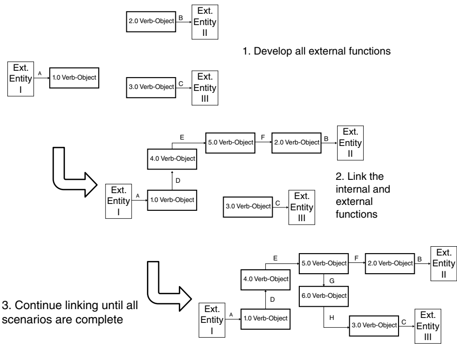
Figure 7.8. Functional block diagram development from external view first.
