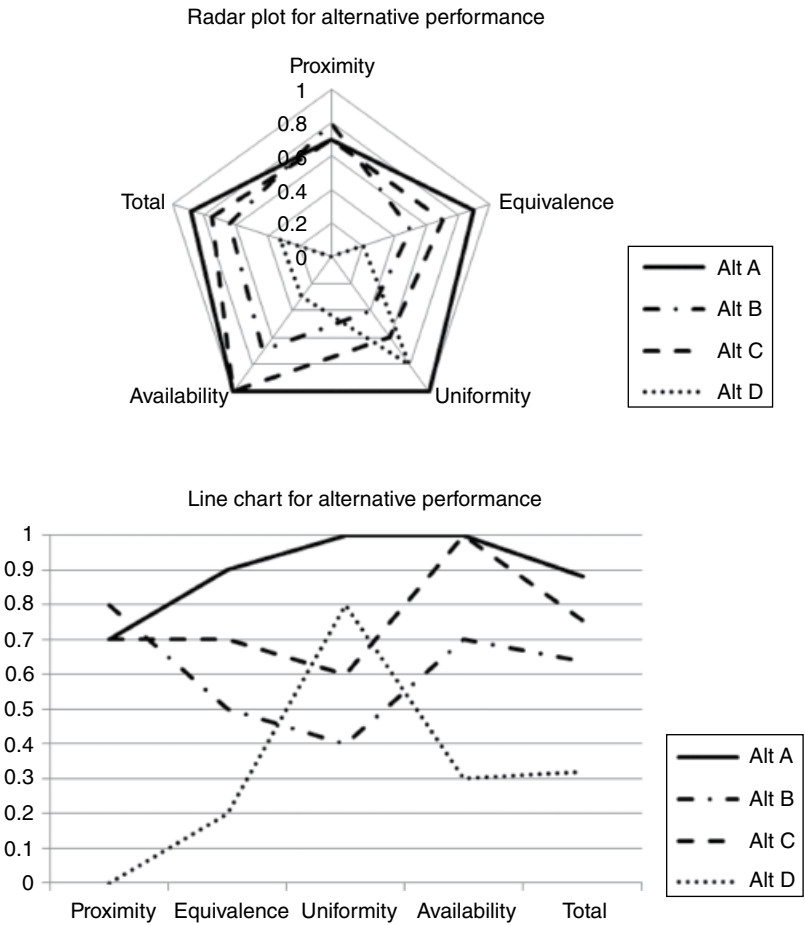
Figure 11.11. MAUT final analysis example plot.
