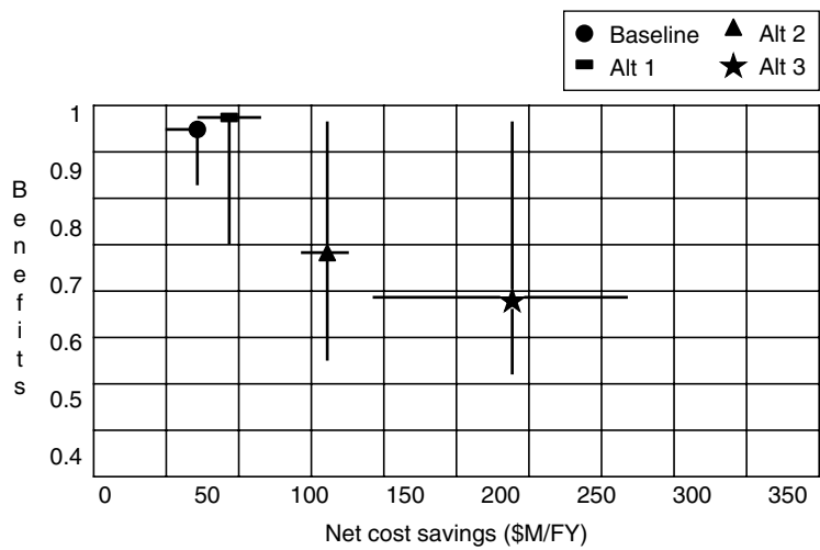
Figure 8.6. Scatterplot of performance and cost comparison.
