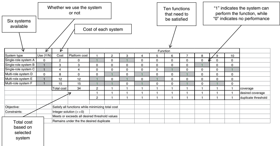
Figure 8.1. Assignment problem to minimize number of machines used.
