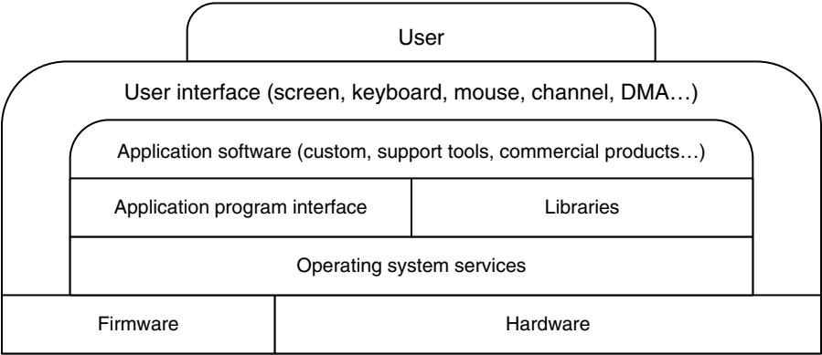
Figure 14.2. Software hierarchy.
